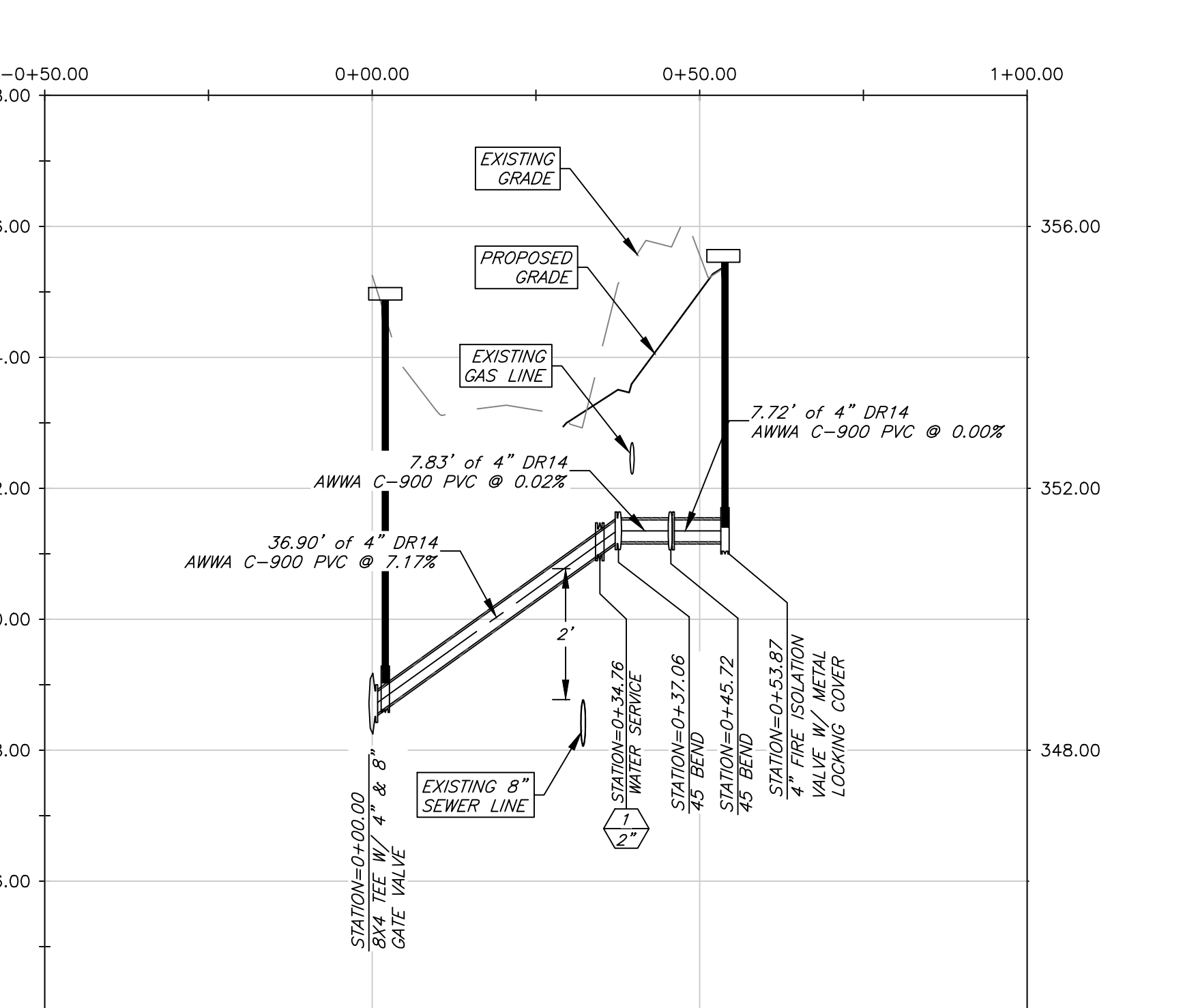
Profile: 4" Waterline -0+50.00 to 1+00.00
